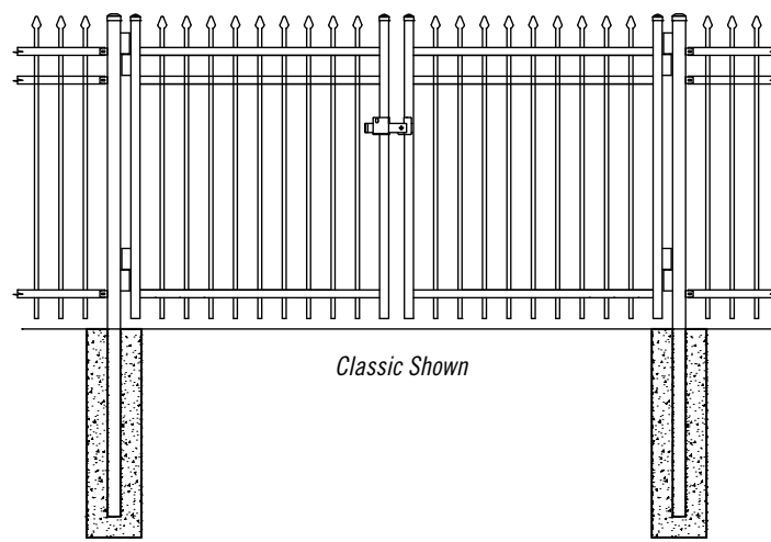
DOUBLE SWING DIMENSIONAL DRAWING
