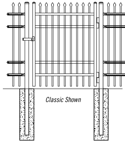
SINGLE SWING DIMENSIONAL DRAWING
