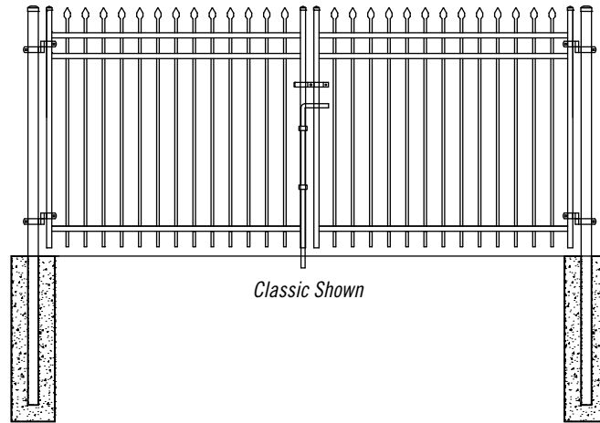
DOUBLE SWING DIMENSIONAL DRAWING
