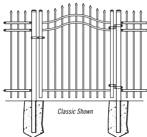
SINGLE SWING DIMENSIONAL DRAWING
